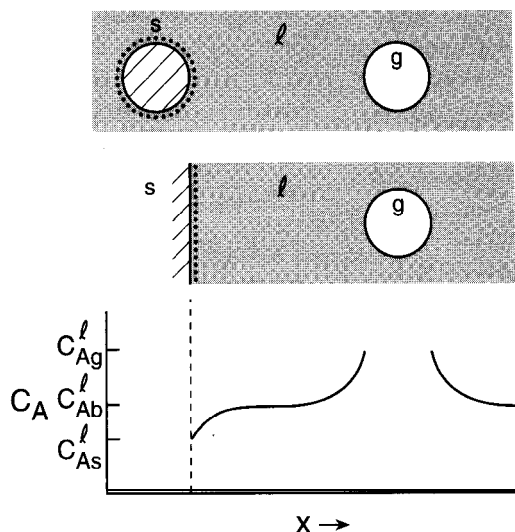
Figure 12-15 Sketch of concentration profiles between a spherical bubble and a solid spherical catalyst particle in a continuous liquid phase (upper) in a gas-liquid slurry reactor or between a bubble and a planar solid wall (lower) in a catalytic wall bubble reactor. It is assumed that a reactant A must migrate from the bubble, through the drop, and to the solid catalyst surface to react. Concentration variations may occur because of mass transfer limitations around both bubble and solid phases.
