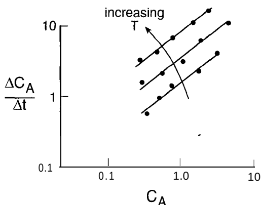
Figure 2-21 Differential reactor data analysis. Plots of \Delta C_A/\Delta t versus C_A on a log-log scale should give straight lines for fixed T . The slope of this line is the order m_A , while the value of the vertical scale where C_A = 1 is the rate coefficient k .
