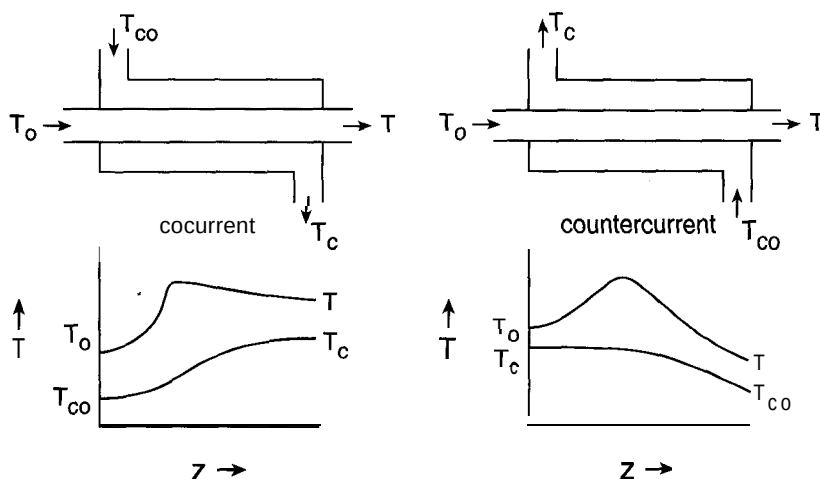
Figure 5-21 Temperature profiles for cocurrent and countercurrent cooled PFTR with feed temperature T_o and coolant feed temperature T_{co} .
