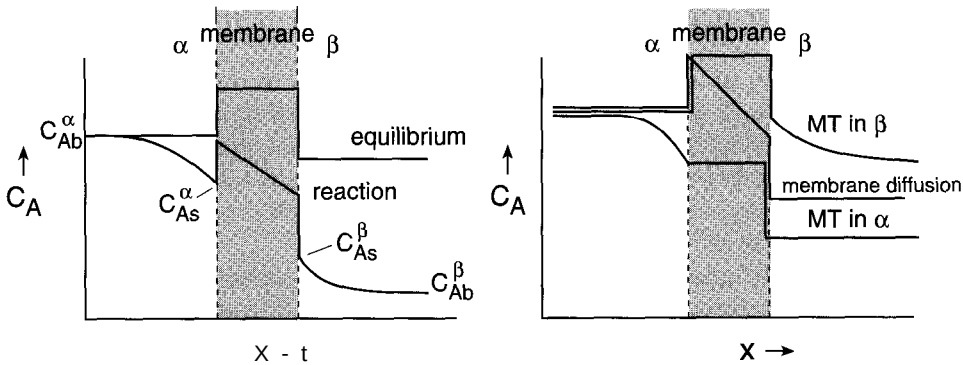
Figure 12-5 Concentration profiles of a reactant that migrates into one phase through a membrane and into a second phase for reaction.
