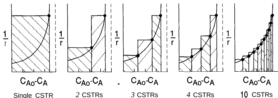
Figure 3-9 Total residence time from 1/r plot for a series of CSTR reactors for 1, 2, 3, 4, and n equal-volume reactors. The total residence time (shaded area) approaches that of a single PFR for large n .
