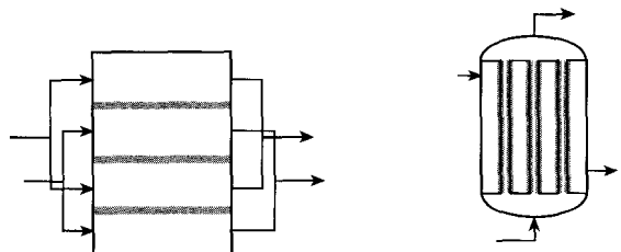
Figure 12-6 Sketches of membrane reactors to attain high areas for transfer of a species.
