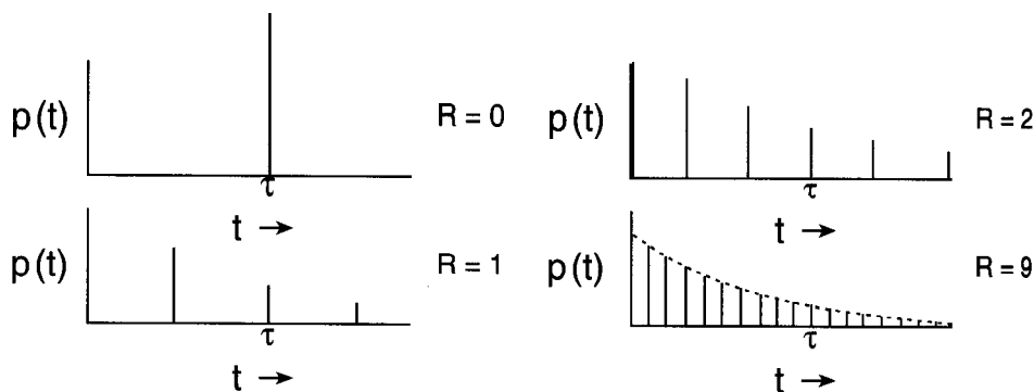
Figure S-11 p(t) for a tubular reactor with increasing recycle.
