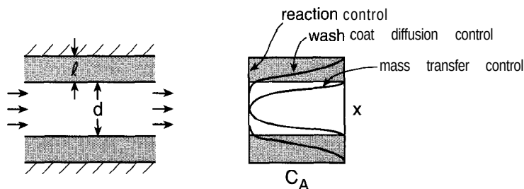
Figure 7-20 Sketch of tube wall reactor with a porous catalyst film of thickness \ell on walls. Expected reactant concentration profiles with reaction-limited, mass-transfer-limited, and pore-diffusion-limited reaction.
