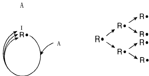
Figure 10-9 Sketch of chain branching reactions where the propagation steps produce more than one radical so that the process tends to grow exponentially, leading to a rapid acceleration of the reaction and possibly a chain-branching explosion.
