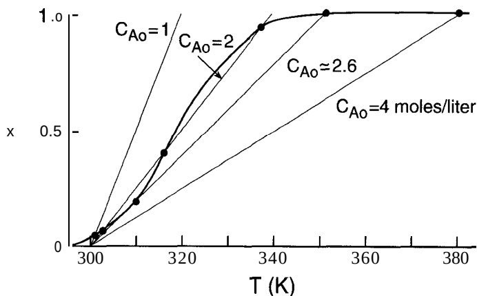
Figure 6-11 Possible multiple steady states in an adiabatic CSTR for variations in the feed concentrations C_{A0} . For low C_{A0} the conversion is low, while for C_{A0} > 2.6 moles/liter only the high conversion steady state can exist. For a range of C_{A0} , three steady states are possible.
