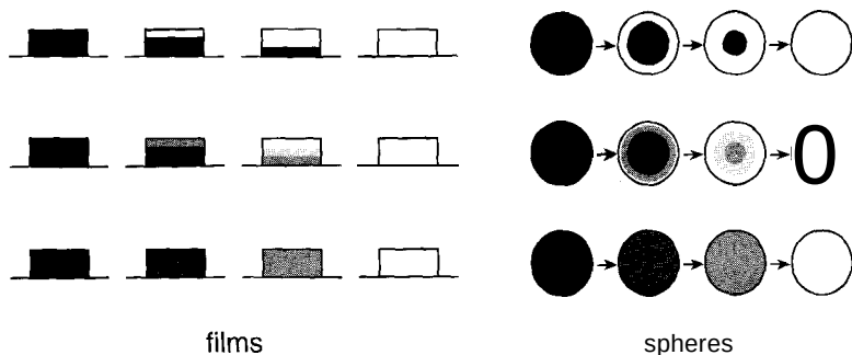
Figure 9-6 Sketches of transforming films or particles, where solid B_s (black) is transformed into C_s (colorless). Sketches shown involve a sharp boundary between reacted and unreacted layers, with reaction assumed to occur only at the interface between the core B and the film C .
