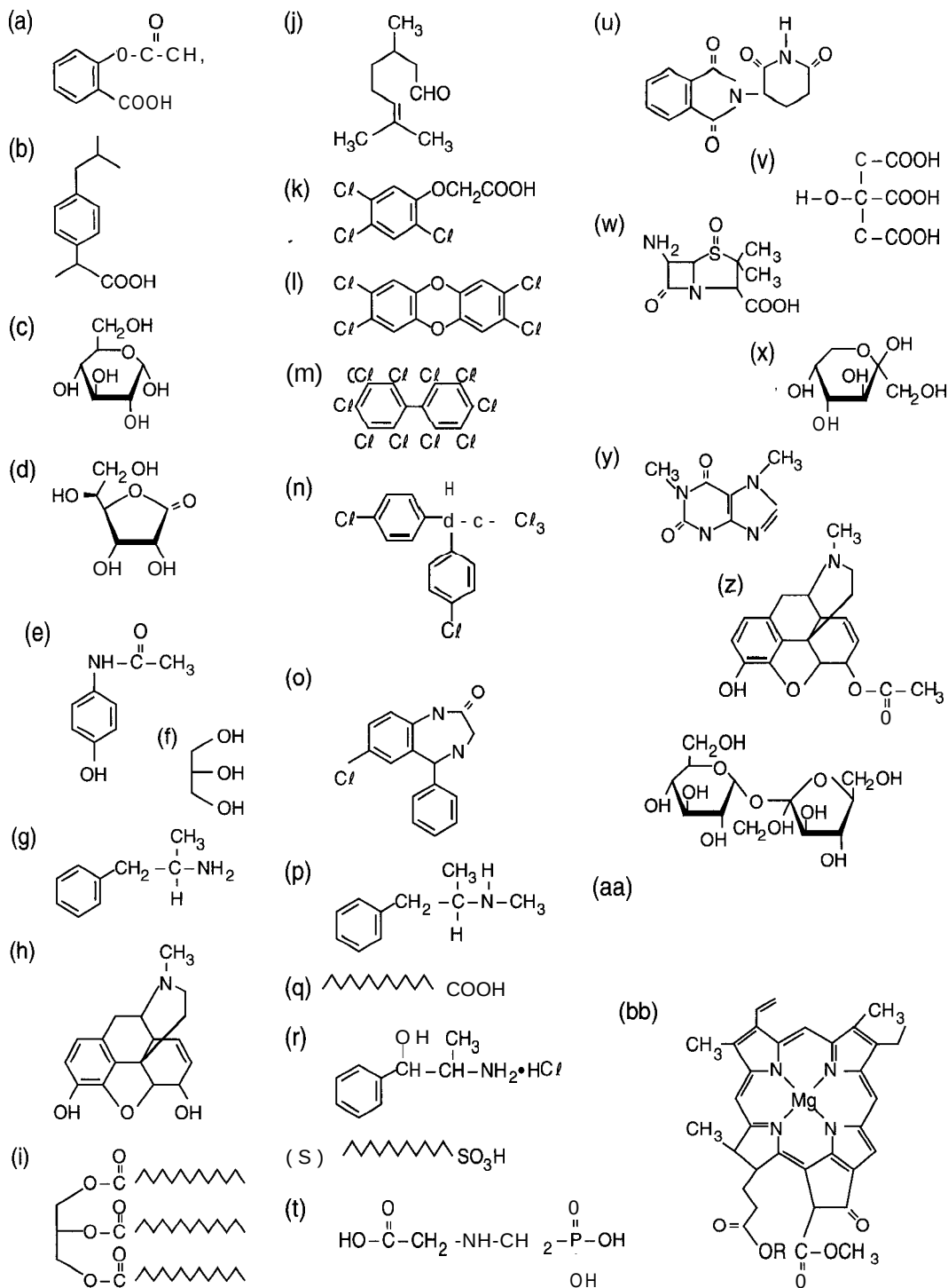
Figure I-I Some very important organic chemicals that are either made in nature or by us.
